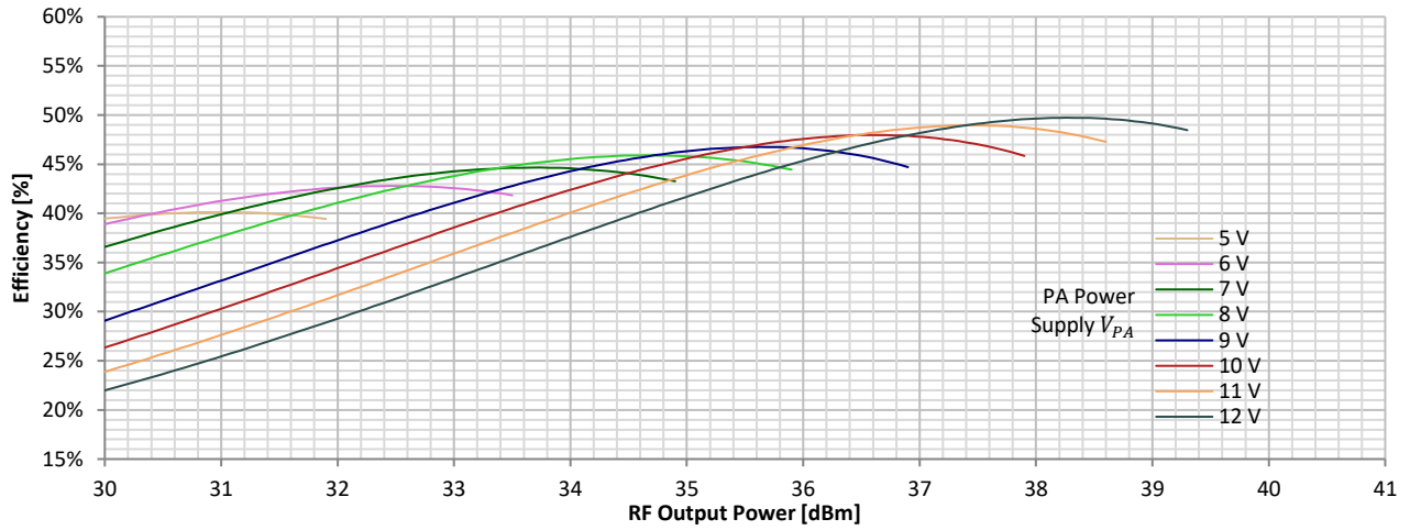
Figure 11 RF Efficiency versus RF Output Power @ 445 MHz
