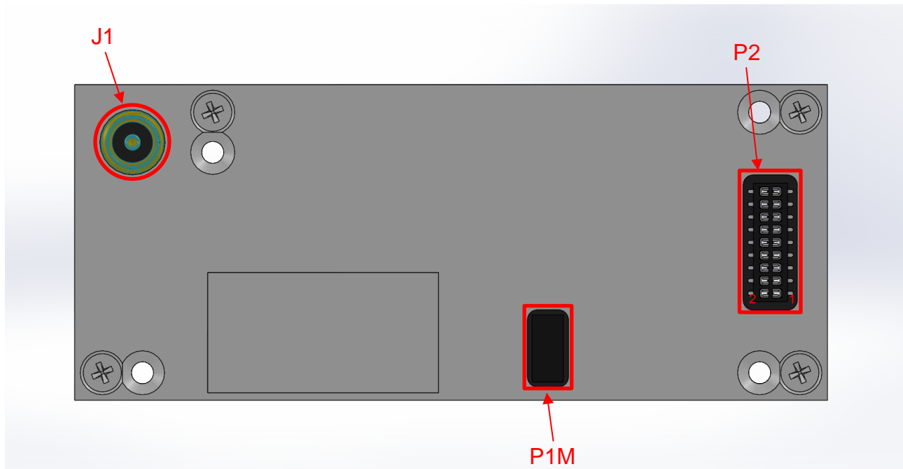
Figure 6 GAUSS High Power UHF Radio Available ports
