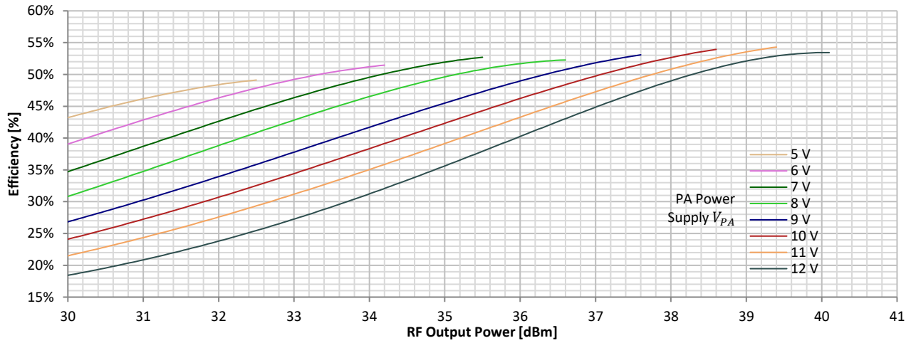
Figure 8 RF Efficiency versus RF Output Power @ 400 MHz
