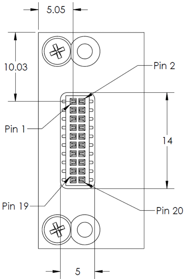
Figure 17 High Power UHF Radio Top Detail B (P2 Connector)
