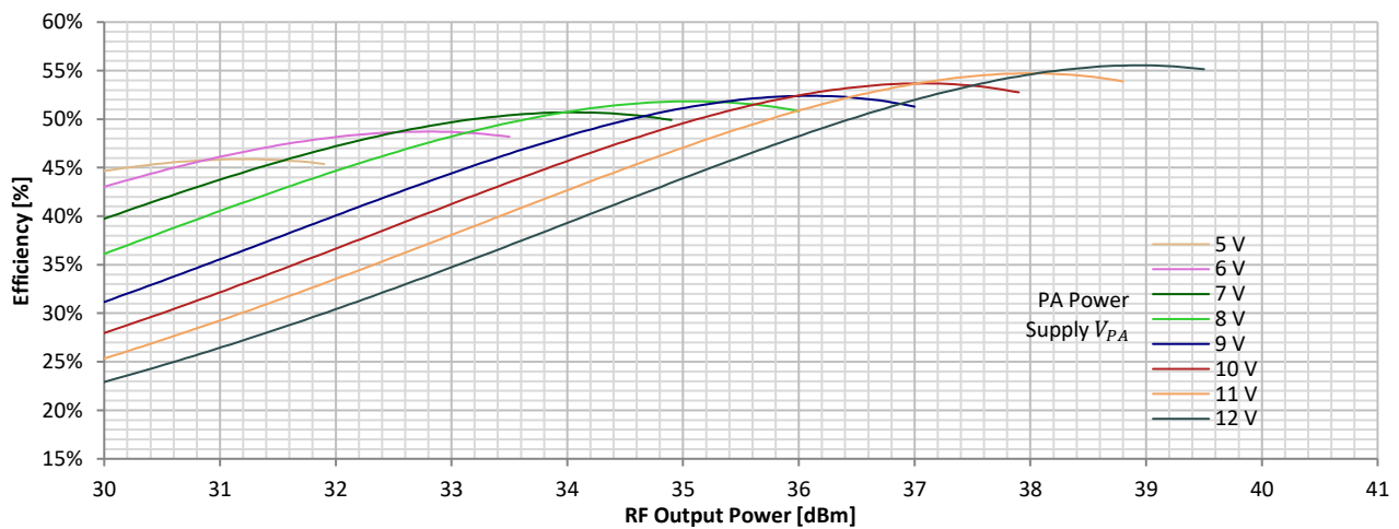
Figure 10 RF Efficiency versus RF Output Power @ 430 MHz
