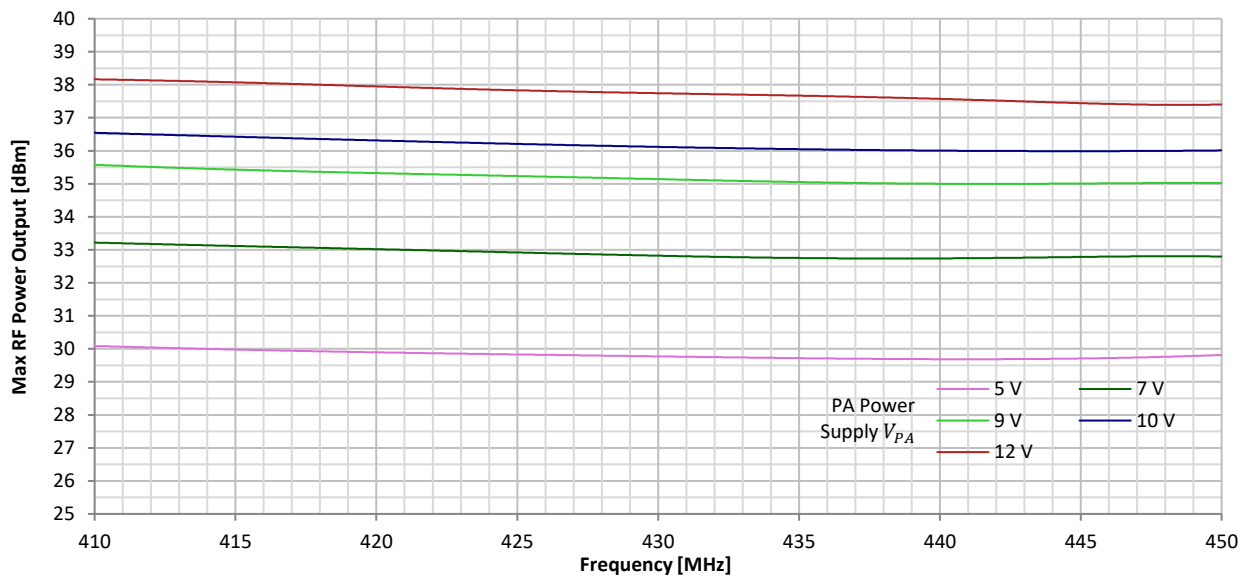
Figure 12 Maximum RF Power Output versus Frequency
