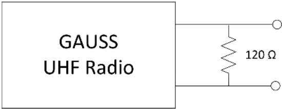
Figure 7 GAUSS High power UHF Radio CAN Bus Termination
