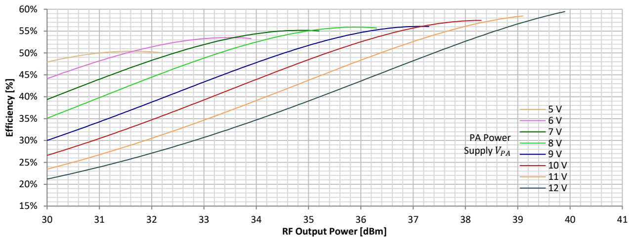
Figure 9 RF Efficiency versus RF Output Power @ 415 MHz
