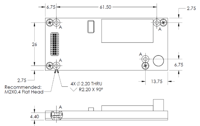
Figure 15 High Power UHF Radio Mounting Details
