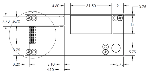
Figure 14 High Power UHF Radio Connectors and Features Top View
