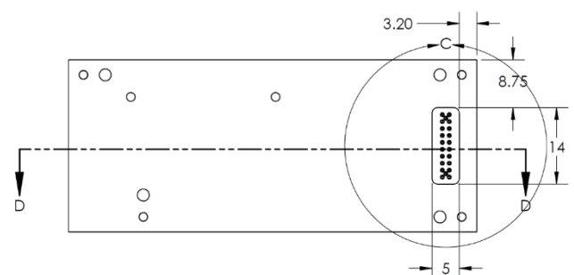
Figure 16 High Power UHF Radio Connector and Features Bottom View
