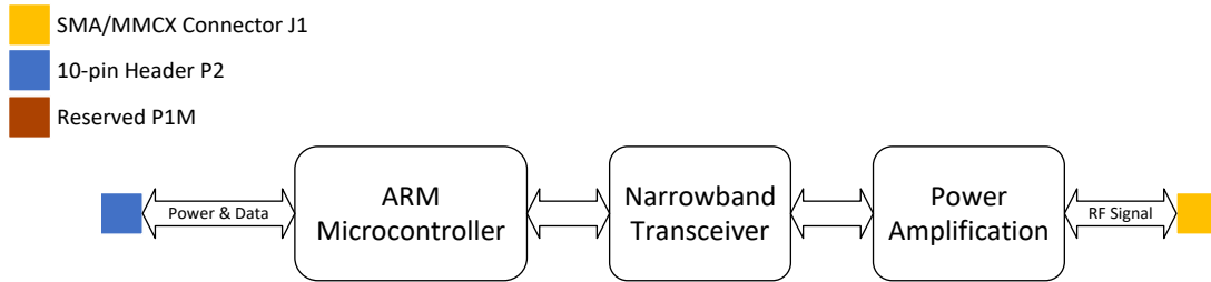
Figure 5 GAUSS High Power UHF Radio General Overview
