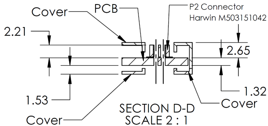
Figure 19 High Power UHF Radio Connectors and Features Section D-D
