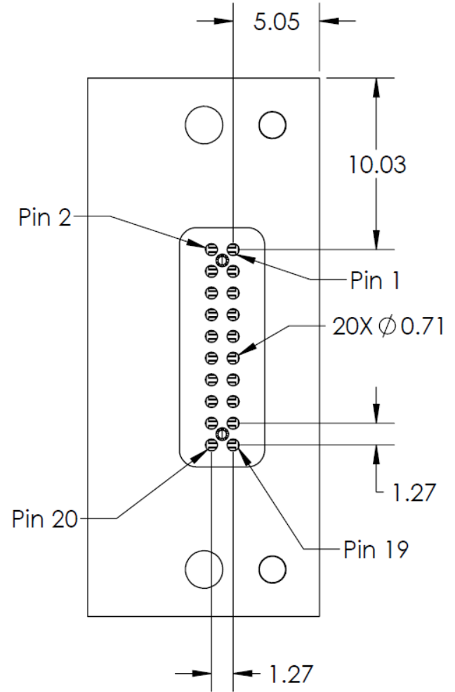
Figure 18 High Power UHF Radio Bottom Detail C (P2 Connector)
