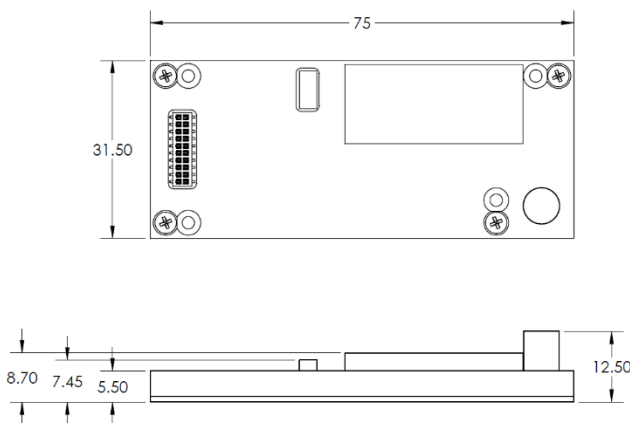
Figure 13 High Power UHF Radio Outer Dimensions
